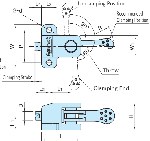
Clockwise Clamping
